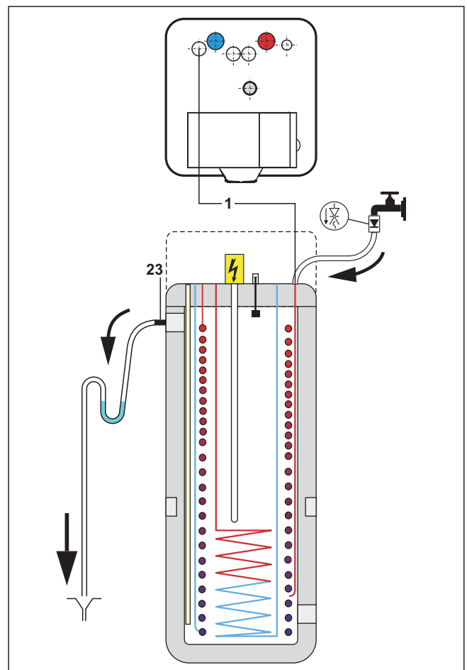
Fig. 8-1 Filling the storage tank - without solar system
