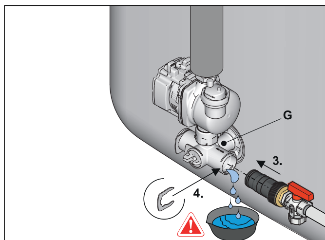
Fig. 5-6 Installing the KFE filling connection in the connection bracket
