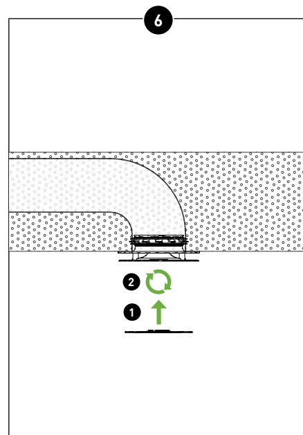
Turn and click the finishing plate onto the vent
