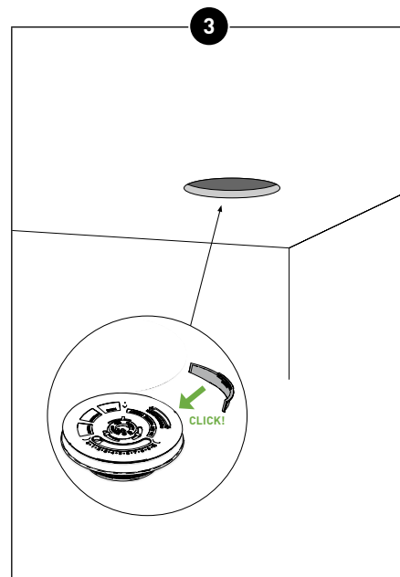
Mounting flow control plate (if <20 cm from wall or corner)
